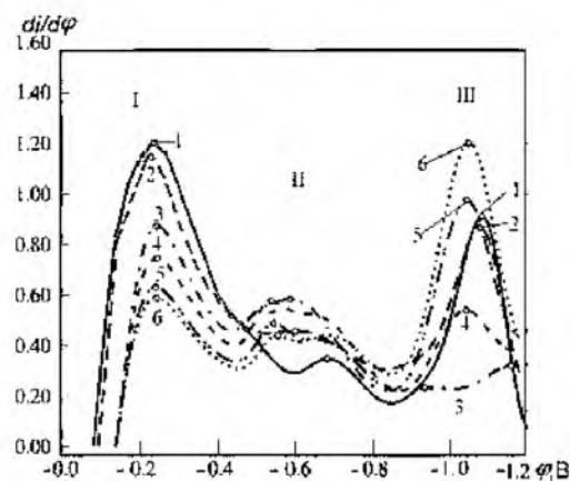
Fig. 5. Differential volt-ampereograms of reduction of free oxygen radicals on a copper cathode against a background of 0.1 M NaCl in water (1) in the presence of various concentrations of GSH (T = 298 K): 2 – 0.24; 3 – 0.47; 4 – 0.74; 5 – 0.91; 6 – 1.1 \cdot 10^3 M/ml
