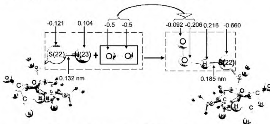
Fig. 2. Scheme of interaction of GSH molecule with \bullet\text{OO}^- (arrows point to charges on atoms according to Lyovdin)
