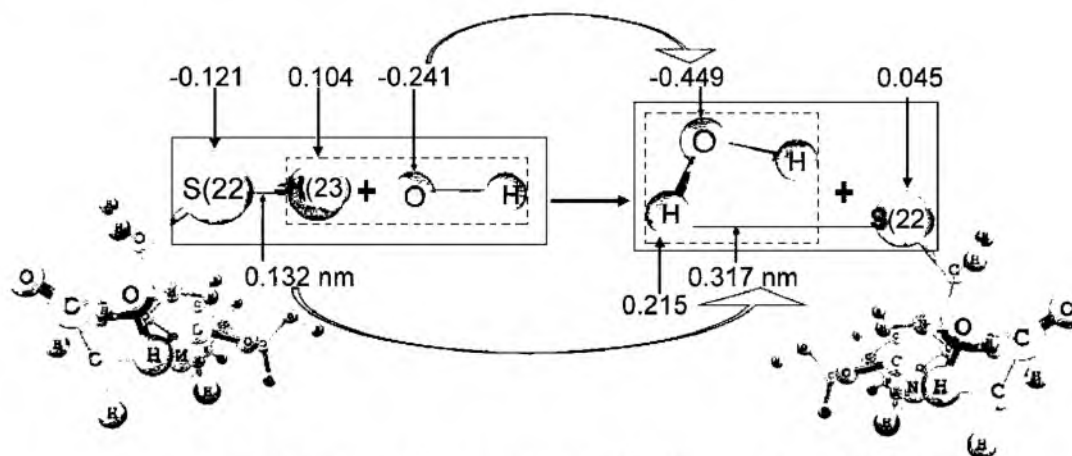
Fig. 3. Scheme of interaction of GSH molecule with \bullet\text{OH} (arrows point to charges on atoms according to Lyovdin)
